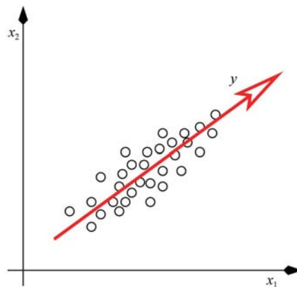
Figure 3 Principal component analysis of a two-dimensional ( x_1, x_2 ) data set. The line labelled y shows the direction of the first principal component, which gives the best mean-square reduction of the data from two to one dimensions.
